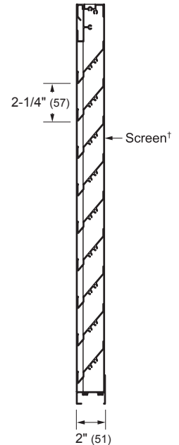
Vertical Section
