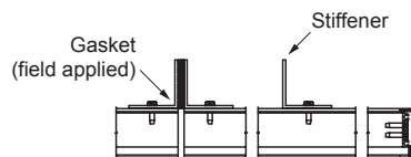
Hidden Vertical Mullion (optional)
