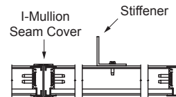
Visible Vertical Mullion (standard)
