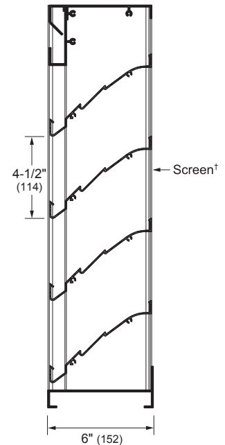
Vertical Section
