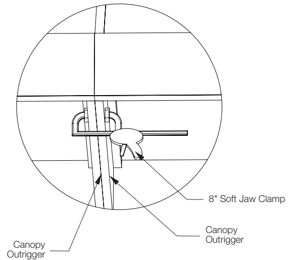
Fig. 3.4 Canopy Clamping
