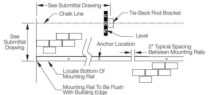
Fig 1.1 Mounting Rail
