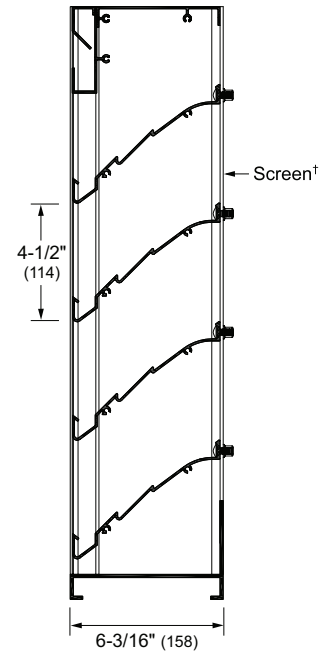
Vertical Section
