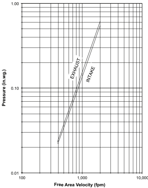
Louver Test Size = 48" x 48" (1219 x 1219)
