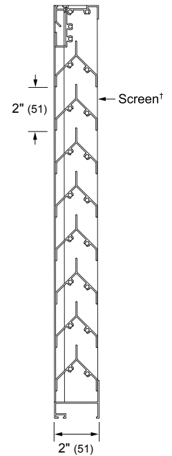
Vertical Section
